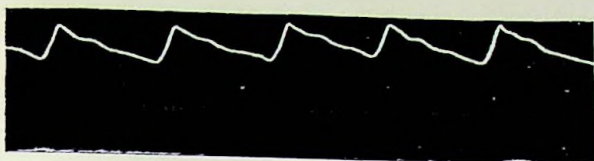
FIG. 10.—Normal pulse.
