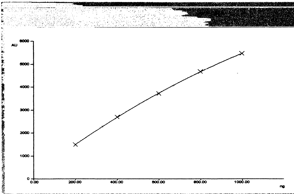
Figure 6: Calibration Curve of Brucine in Mkted Samples & Std. MQ (area)
