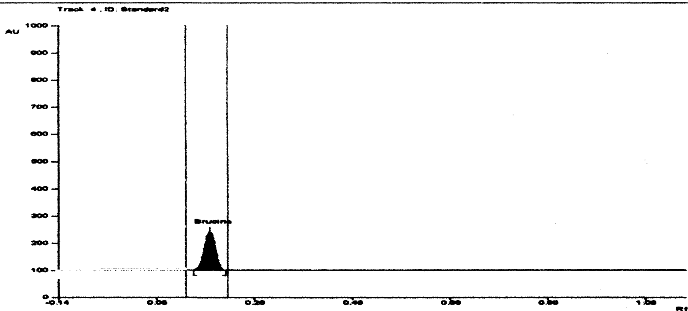
Figure 3: Chromatogram of Std. Brucine (Rf = 0.18)
