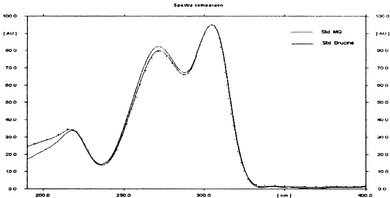
Figure 5: Overlay of Absorption Spectra of Std. Brucine and its Corres. Fraction in Std. MQ
