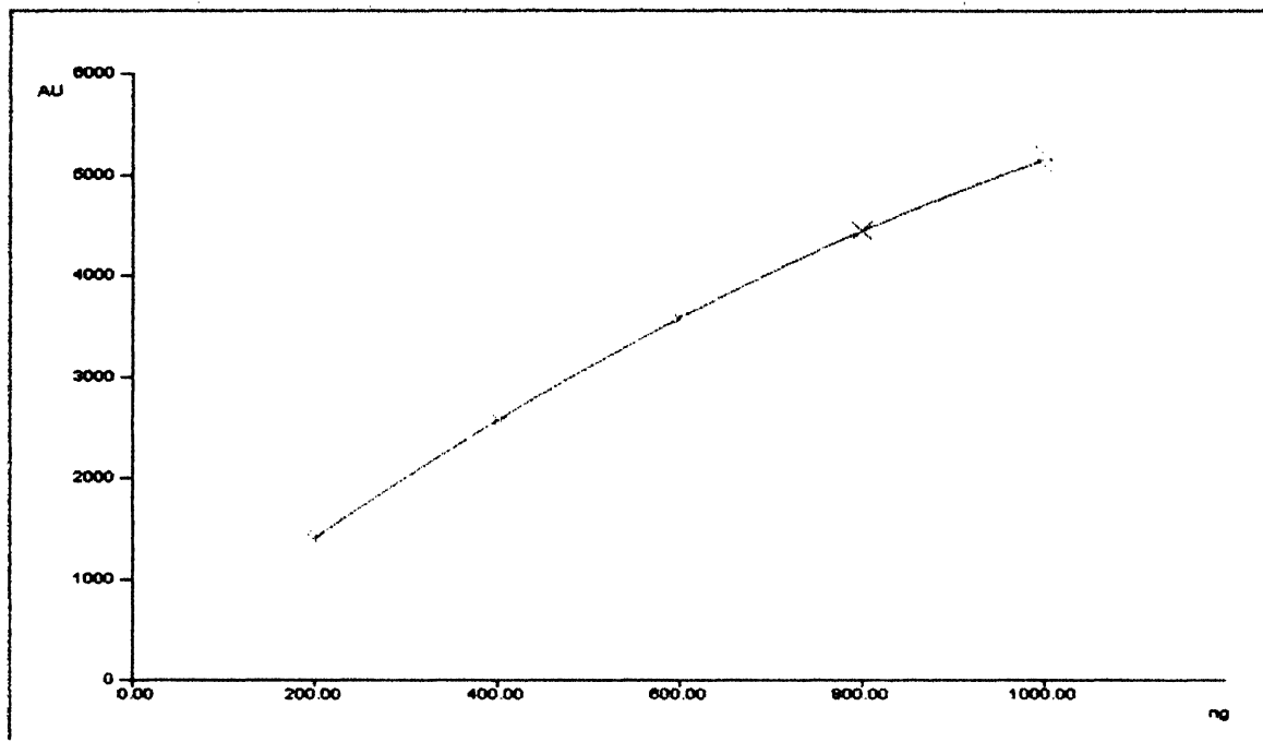
Figure 4: Calibration Curve of Brucine (area)
